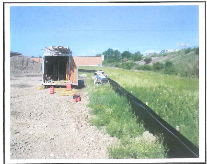
Silt fence maintained between project and stormwater swale.
